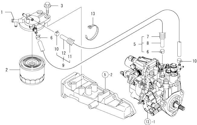
Fig.16. FUEL LINE
