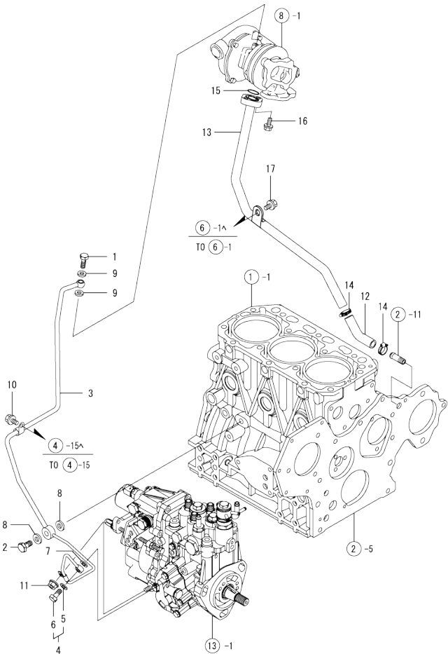
Fig.11. LUB.OIL LINE
